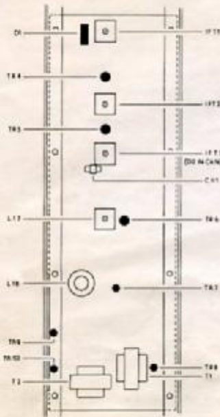
Layout of IF Printed Board
